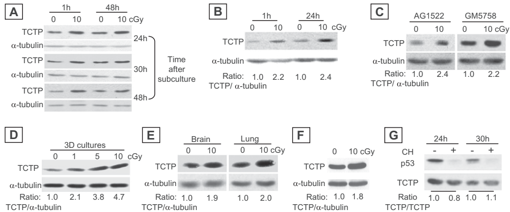
Fig. S1. Western blot analyses of translationally controlled tumor protein (TCTP) in normal human cells and in tissues of mice exposed to low-dose ^{137}\text{Cs} \gamma rays or 1 GeV protons. (A) Up-regulation of TCTP in asynchronous cells. Confluent normal human AG1522 cells were subcultured and exposed to acute \gamma rays at different time points: 24 h later, when the population was enriched in S-phase cells; at 30 h, when the population was enriched in G_2/M cells; and at 48 h, when dividing cells progressed in the following growth cycle. Cells were harvested 1 or 48 h after irradiation, and TCTP expression was quantified. (B) TCTP was induced up to 24 h after exposure of confluent AG1522 cells to acute 10 cGy of \gamma rays. (C) TCTP expression in confluent AG1522 or GM5758 normal human skin fibroblasts at 4 h after no exposure or acute exposure to 10 cGy of \gamma rays. (D) TCTP up-regulation in irradiated AG1522 cells maintained in a 3D architecture. Cells were exposed to low-dose \gamma rays and harvested 4 h later. (E) TCTP is up-regulated in tissues of C3H/HeJ mice exposed to whole-body irradiation by low-dose \gamma rays. Tissues were harvested for analysis 4 h after exposure. (F) TCTP is up-regulated in confluent AG1522 cells exposed to 1 GeV protons and harvested 24 h later. (G) Western blot analyses of TCTP in AG1522 confluent cell cultures exposed to 10 cGy irradiation at an acute dose rate (6 cGy/min) in the presence or absence of cycloheximide (2 \mu\text{g}/\text{mL} ). Cells were incubated in cycloheximide for 30 min before irradiation and were harvested for analysis 24 or 30 h later.
